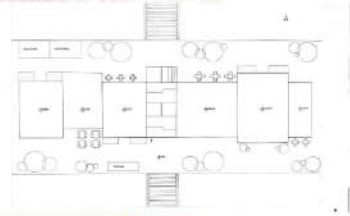
Yatay Plan
